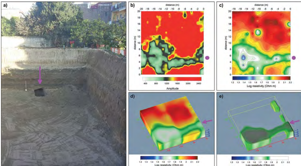
Fig. 10 – a): an unknown tunnel in the area of Pomigliano d'Arco (Naples, Italy); b): GPR horizontal section relative to 1.5 m in depth; c): ERT horizontal section relative to 1.5 m in depth; d): three-dimensional view of the investigated tomospace; e): three-dimensional view of high resistivity values.
