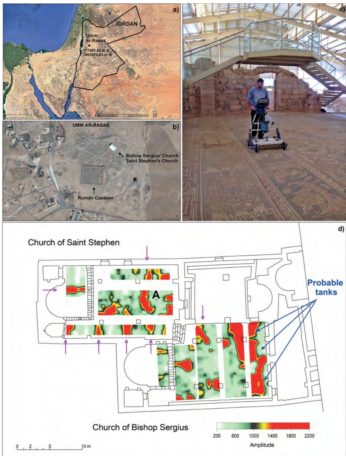
Fig. 3 – a): location of Umm ar-Rasas on a Google Earth™ satellite image of Jordan; b): detail of the site with indication of the roman castrum and the two Byzantine Churches; c): GPR prospection; d): horizontal slices related to the depth window of 0.5-0.7 m overlapped on the map of the churches (the blue arrows indicate the location of probable tanks, while the pink arrows highlight probable buried archaeological structures).
