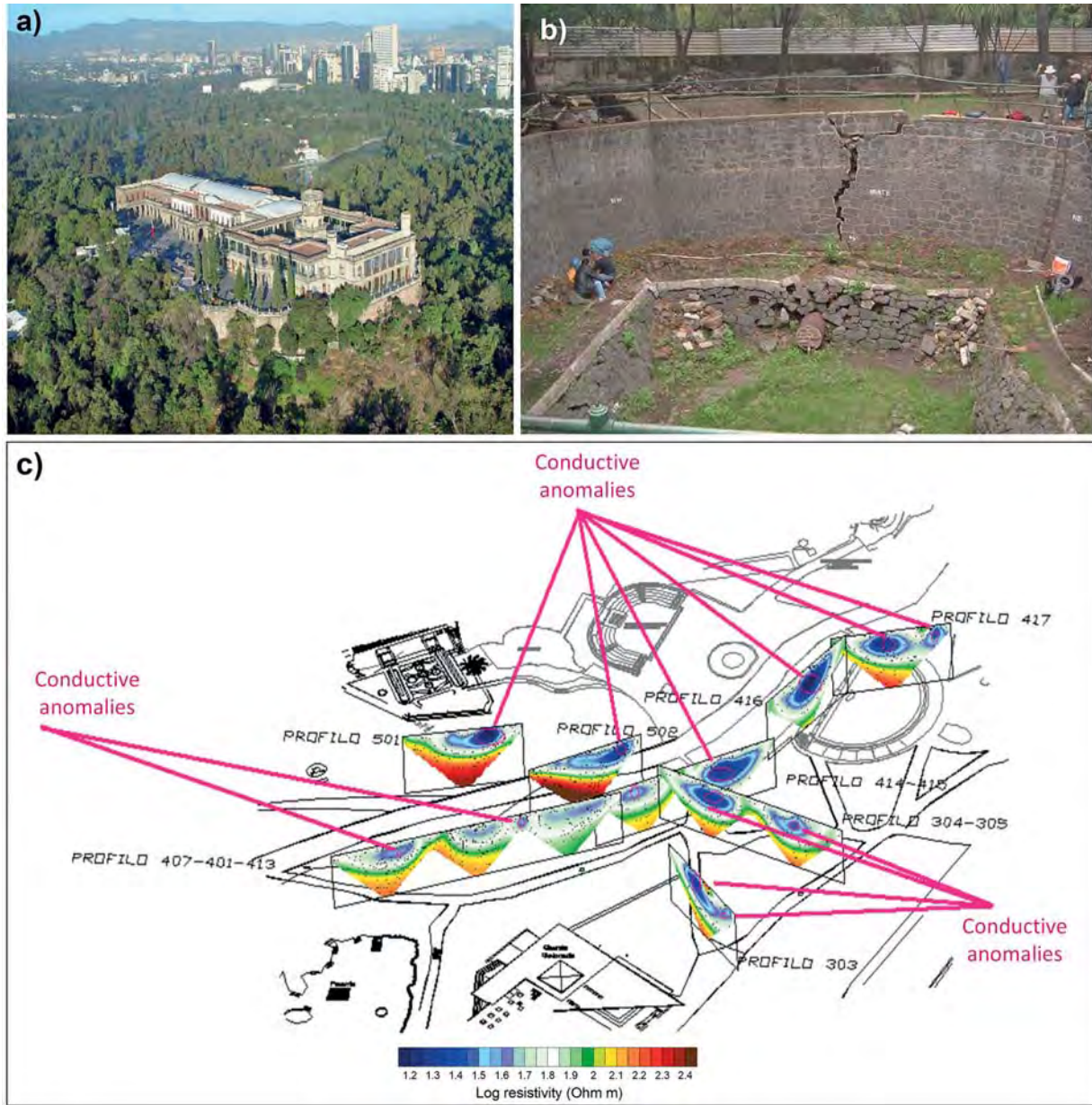
Fig. 4 – The castle of Chapultepec Park (a) and the Bath of Montezuma (b), on the Chapulín hill, Mexico City. The network of water channels as resulting from ERT survey (c).
