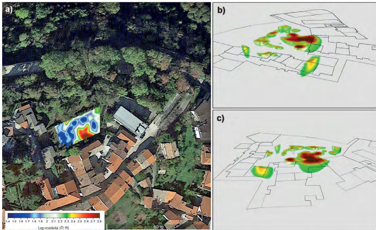
Fig. 2 – a): resistivity map relative to 3 m in depth; b), c): three-dimensional views of the tomospaces.
