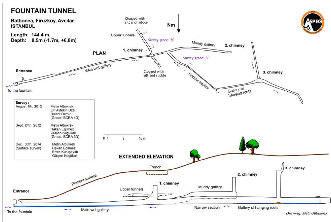
Fig. 4: plan of the Fountain Tunnel.
