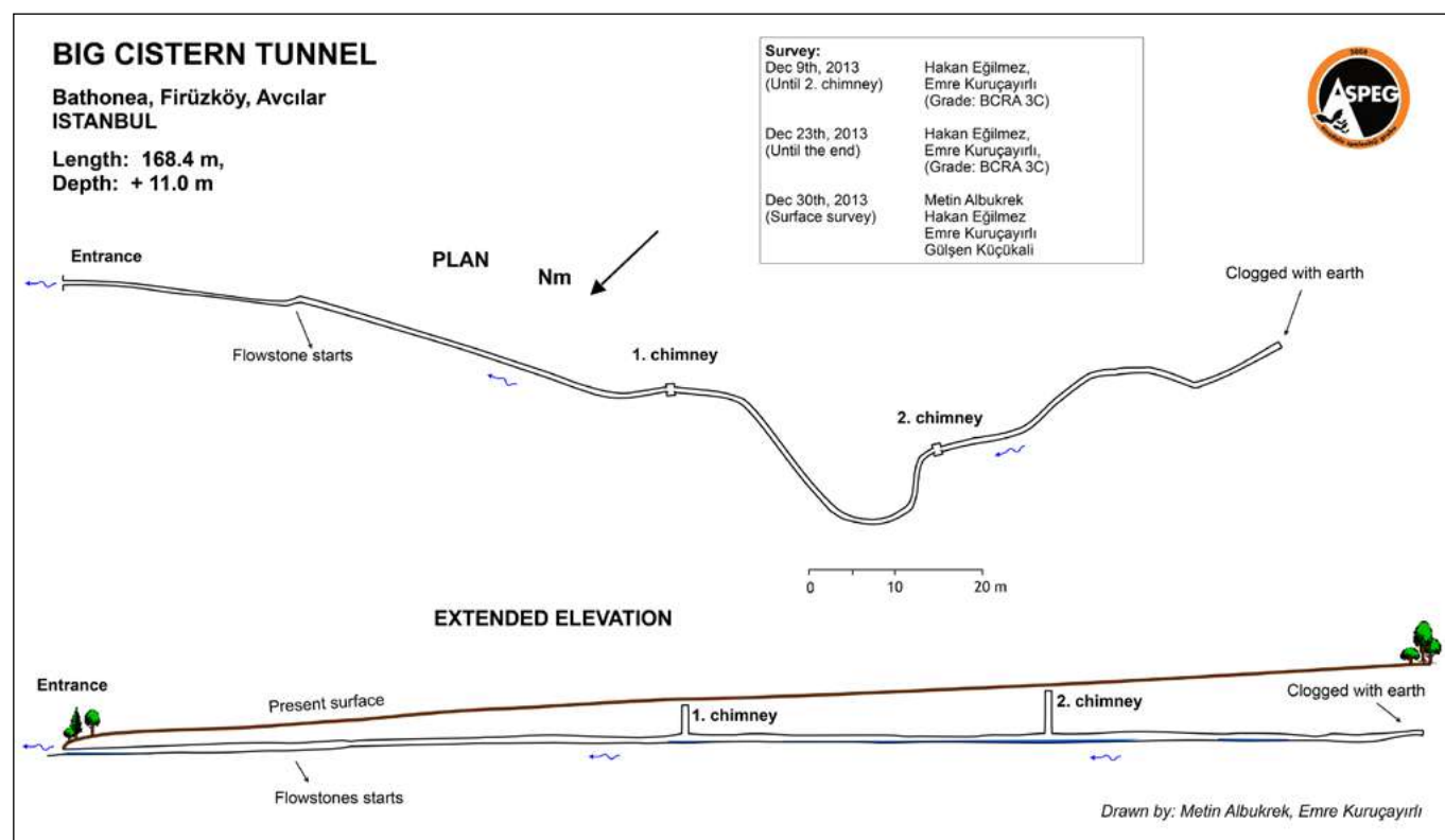
Fig. 11: plan of the Big Cistern Tunnel.
